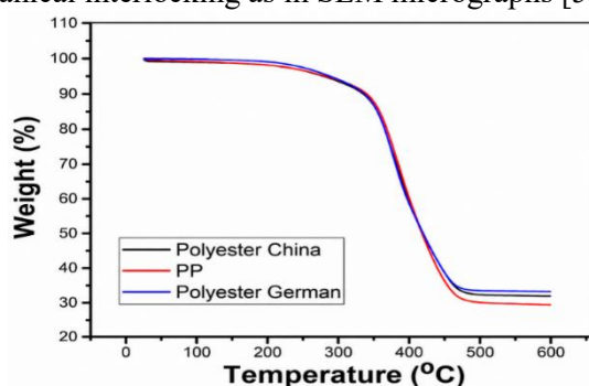
Figure 7. Thermogravimetric curves of RU-Fabric-PU sandwiches with different fabrics
