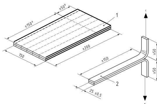
Figure 5. Dimensions of panel samples for the peel strength test [27]
