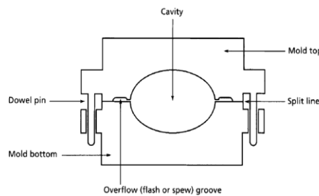
Figure 2. Compression molding
