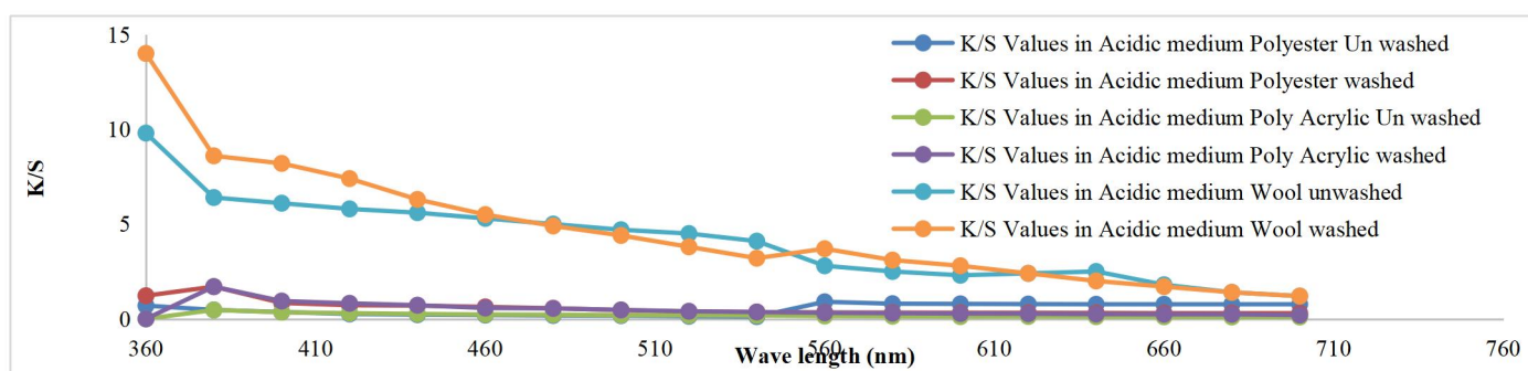
Figure 8: K/S values of unwashed and washed in Acidic medium
