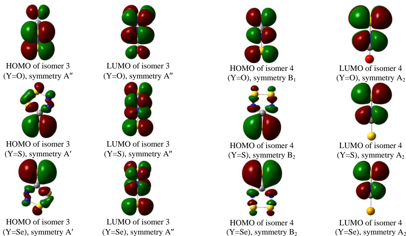
Fig-3(c): Predicted HOMO and LUMO of the ketones for isomer 3
