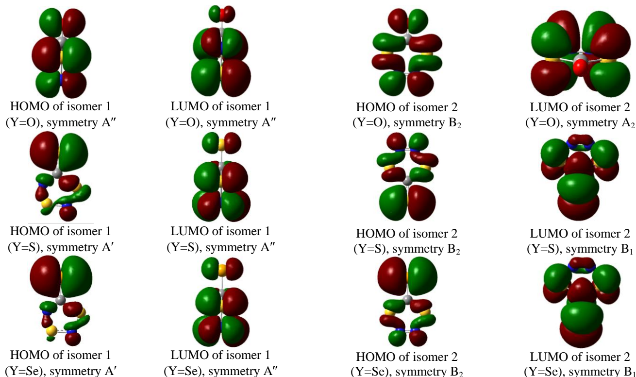
Fig-3(a): Predicted HOMO and LUMO of the ketones for isomer 1
